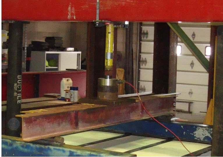
Figure 13. Loading Ram and Load Cell
